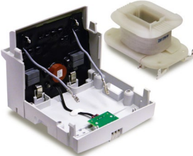
Replacement Coil with EI Interface includes coil, cover and face plate
