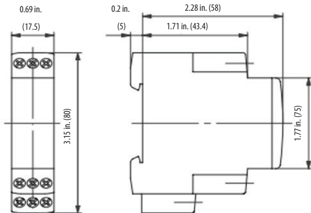
RZ7-FE with 2 c/o Contacts
