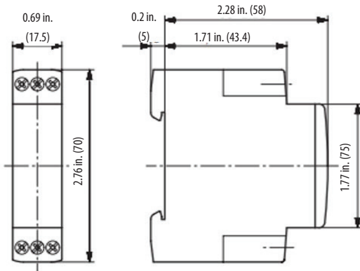
RZ7-FE with 1 c/o Contact or 2 n/o Contacts
